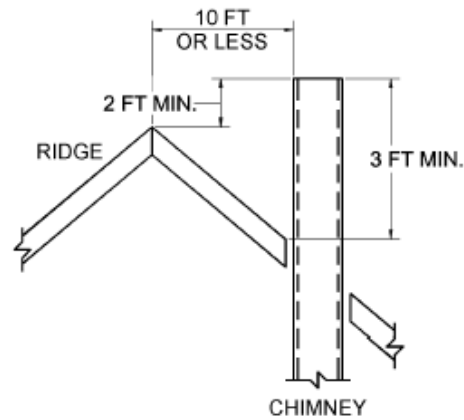
A. TERMINATION 10 FT OR LESS FROM RIDGE, WALL, OR PARAPET
