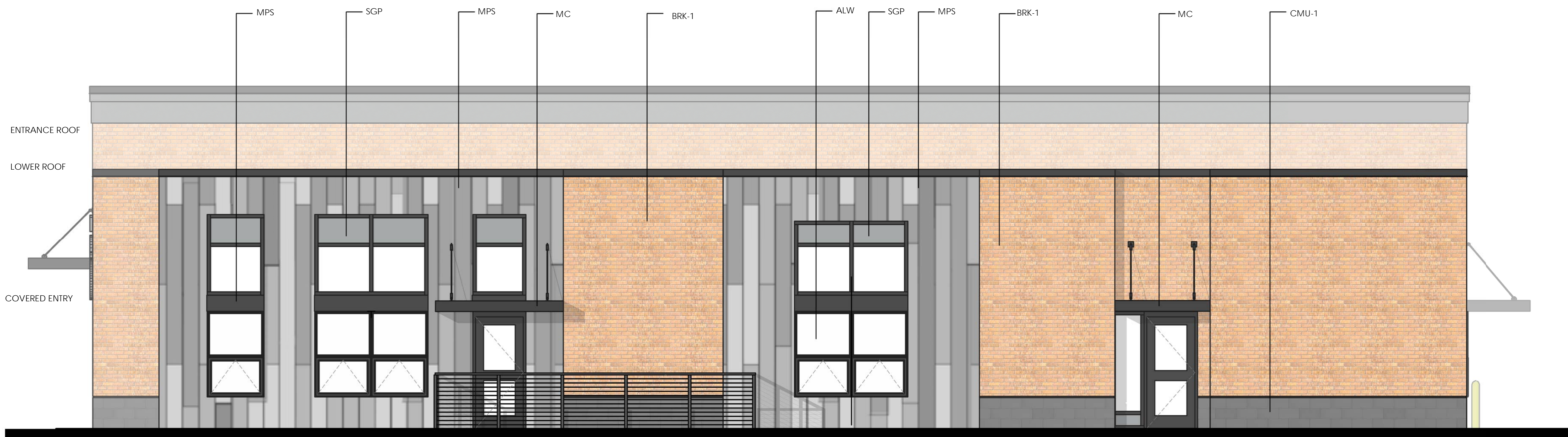
2 EAST ELEVATION 0' 1' 2' 4' 8' 1/4" = 1'-0"
